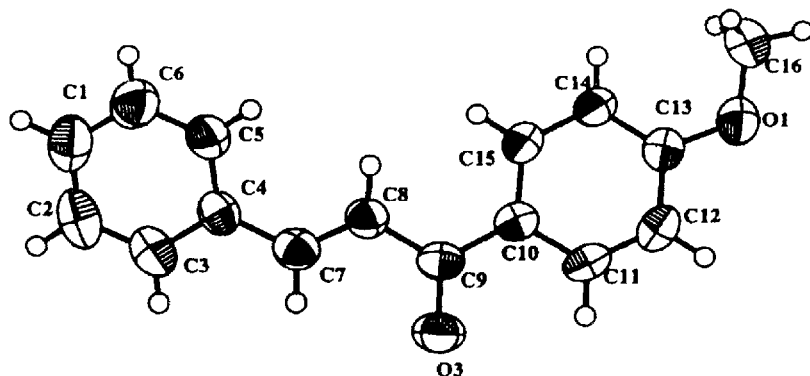
FIGURE 4 ORTEP of the molecule at 50% probability
