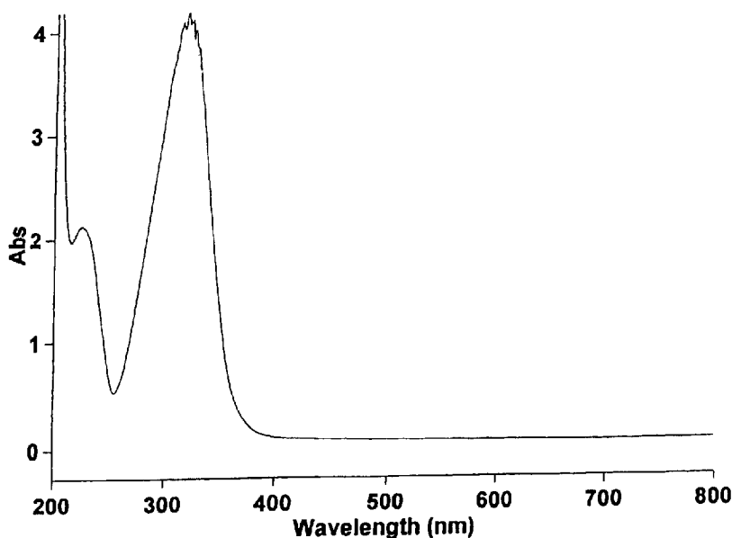
FIGURE 1 UV / Visible spectra
