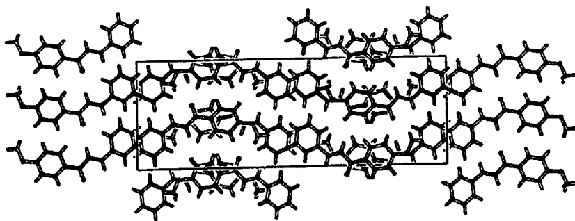
FIGURE 5 Packing of the molecules of down a axis
