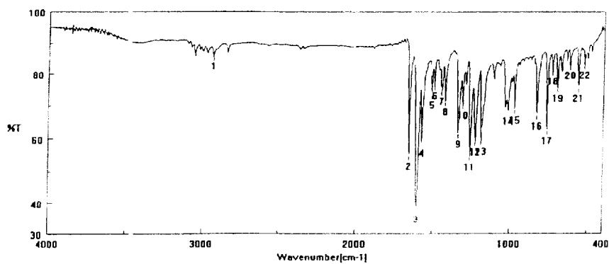
FIGURE 2 IR spectra
