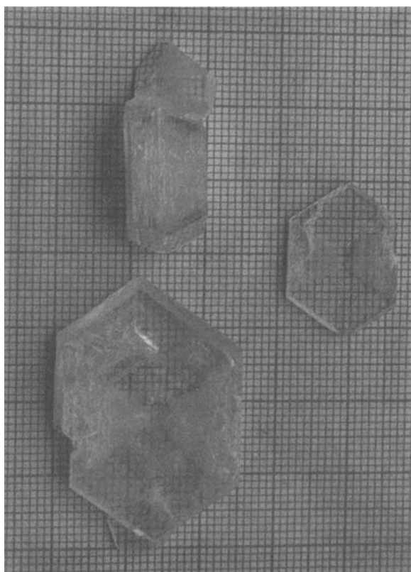
FIGURE 3 Crystal grown in acetone (See Color Plate II at the back of this issue)
